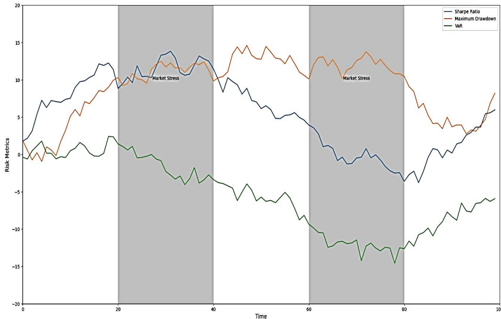
Figure 3: DRL Agent Performance Under Various Risk Scenarios
