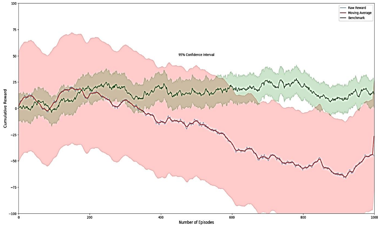
Figure 4: Training Convergence Plot
